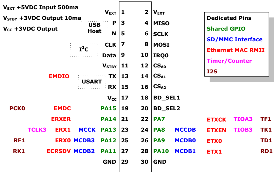
FIGURE 3 Interboard Connector
